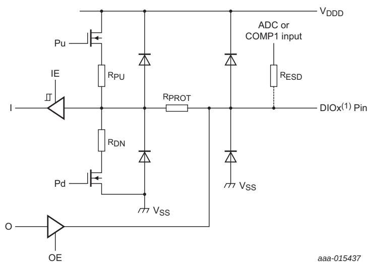
Fig 5. DIO (other than DIO4 and DIO5) pin equivalent schematic
