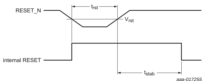
Fig 46. Externally applied reset
