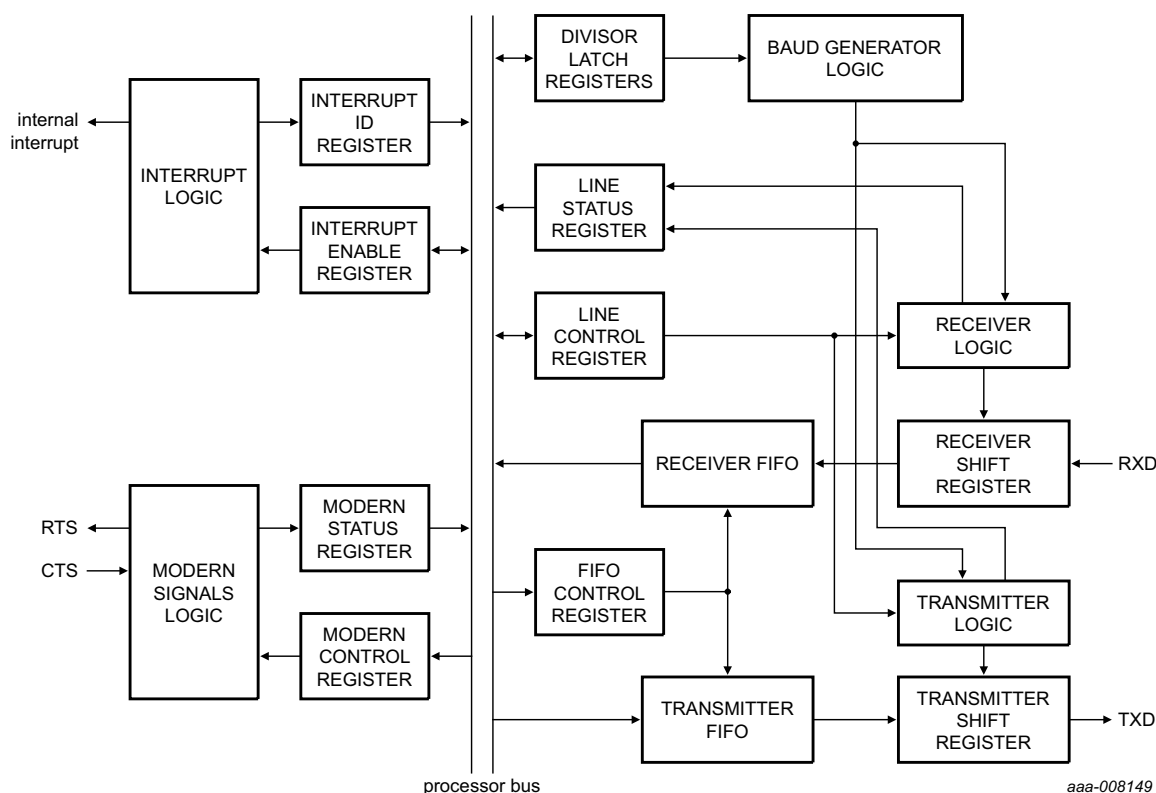
Fig 32. UART block diagram
