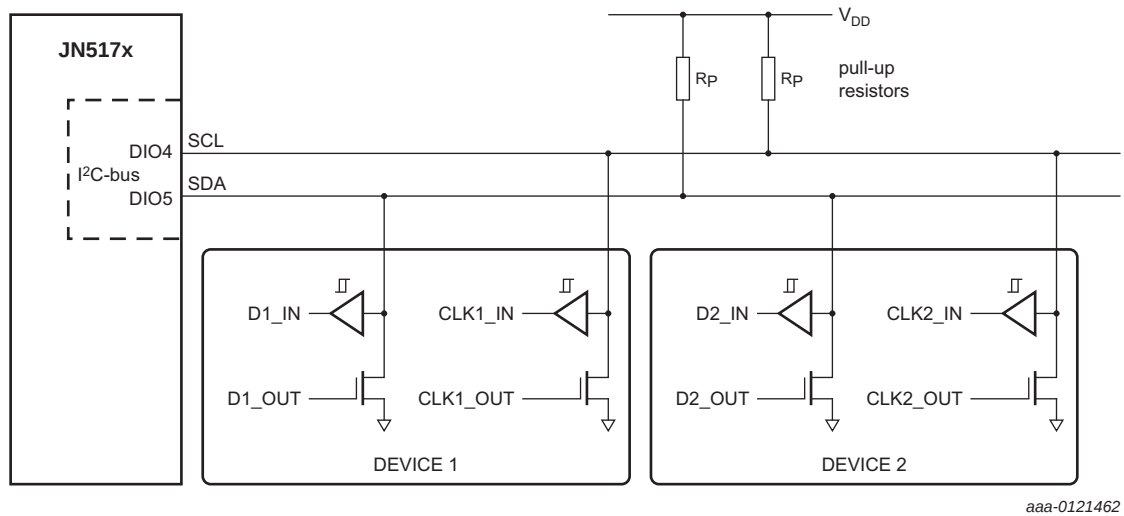
Fig 34. Connection details
