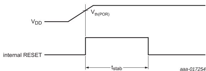
Fig 45. Internal Power-On Reset without showing Brown-Out
