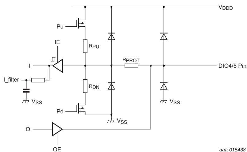
Fig 6. DIO4 and DIO5 pin equivalent schematic
