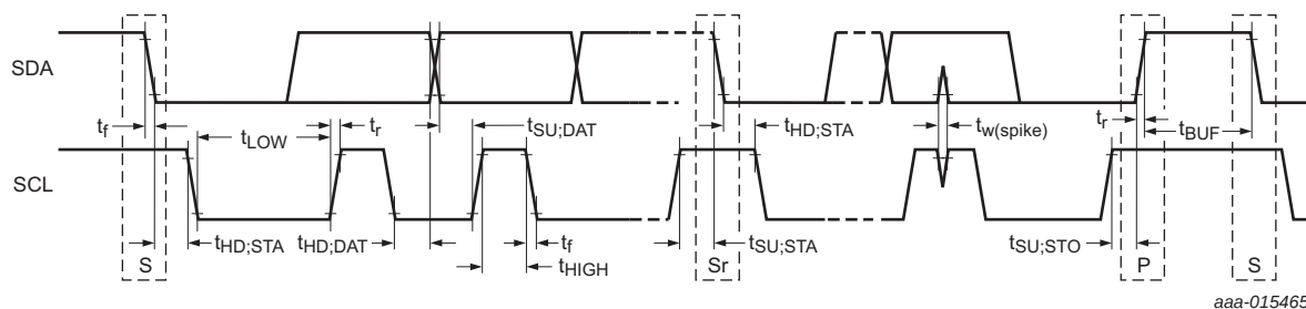
Fig 50. I 2 C-bus interface timing
