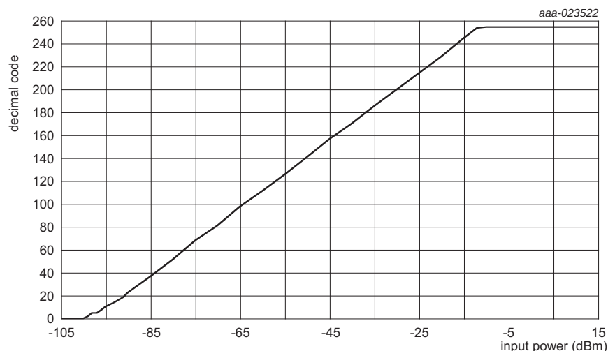
Fig 20. Energy detect value versus receive power level
