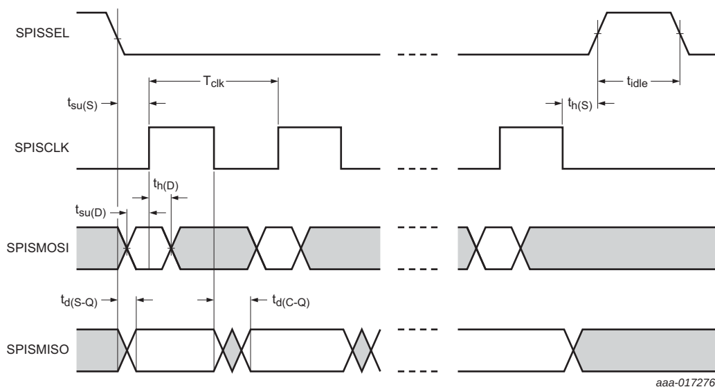
Fig 49. SPI-bus slave timing
