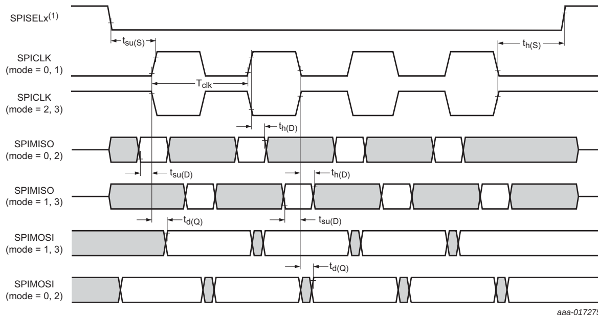
Fig 48. SPI-bus master timing
