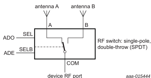
Fig 17. Simple antenna diversity implementation using external RF switch
